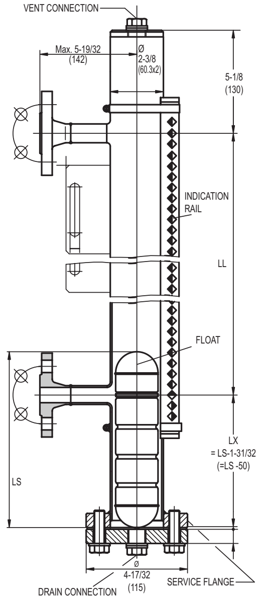
TYPICAL OUTLINE DRAWING
